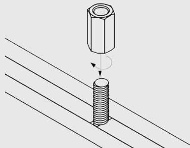
Threaded Rod Attachment
